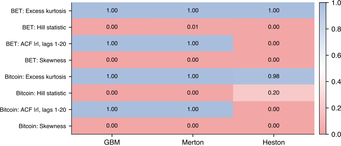
Percentile q of the data in 100 simulated samples
