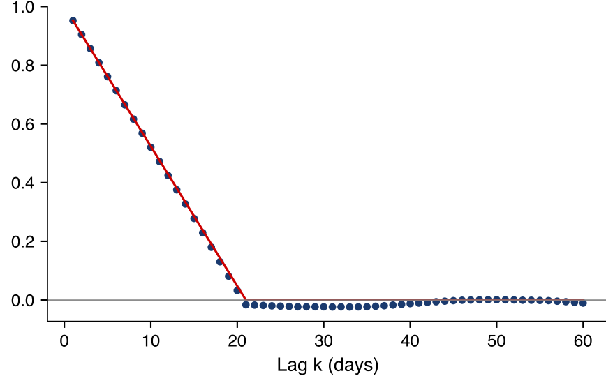
Control: persistence created by the window alone
