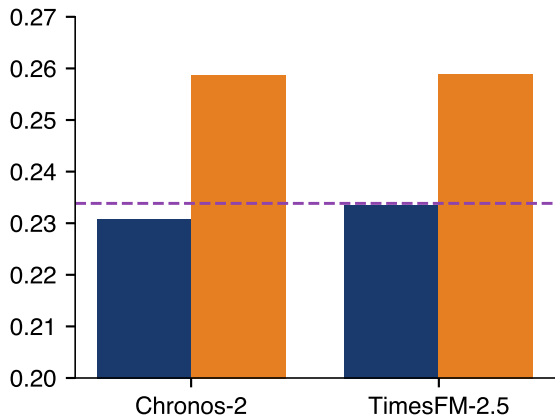
Mean QLIKE
