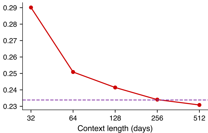
Mean QLIKE
