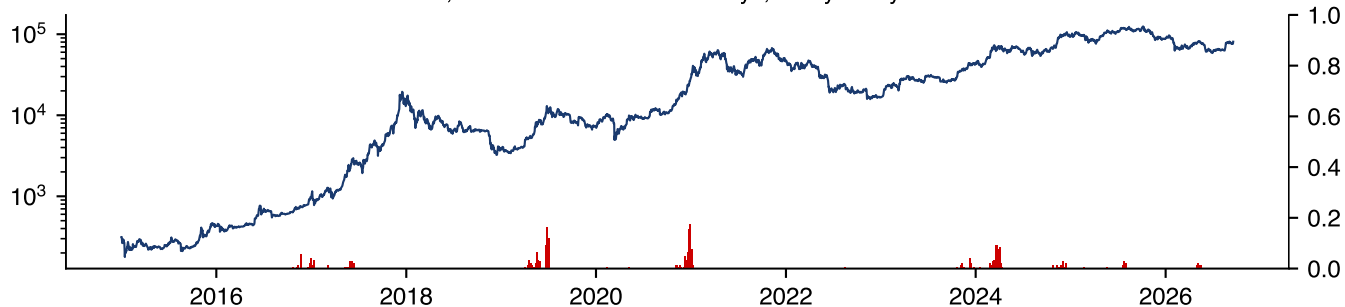
Bitcoin: LPPLS confidence indicator, 141 windows of 50-750 days, every 5 days
