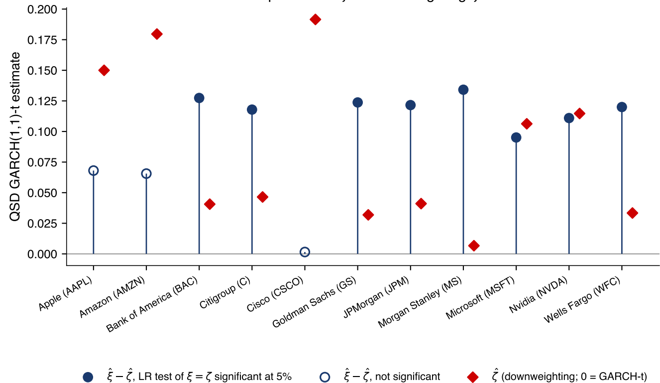
Quasi score-driven GARCH(1,1)-t, 11 S&P 500 stocks, 1995–2019: tail parameter \hat{\xi} vs downweighting \hat{\zeta}
