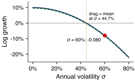
Volatility drag, arithmetic mean 10%
