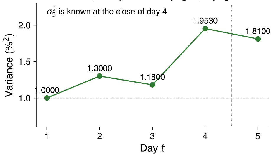
Output: \sigma_t^2 = \omega + \alpha \varepsilon_{t-1}^2 + \beta \sigma_{t-1}^2
