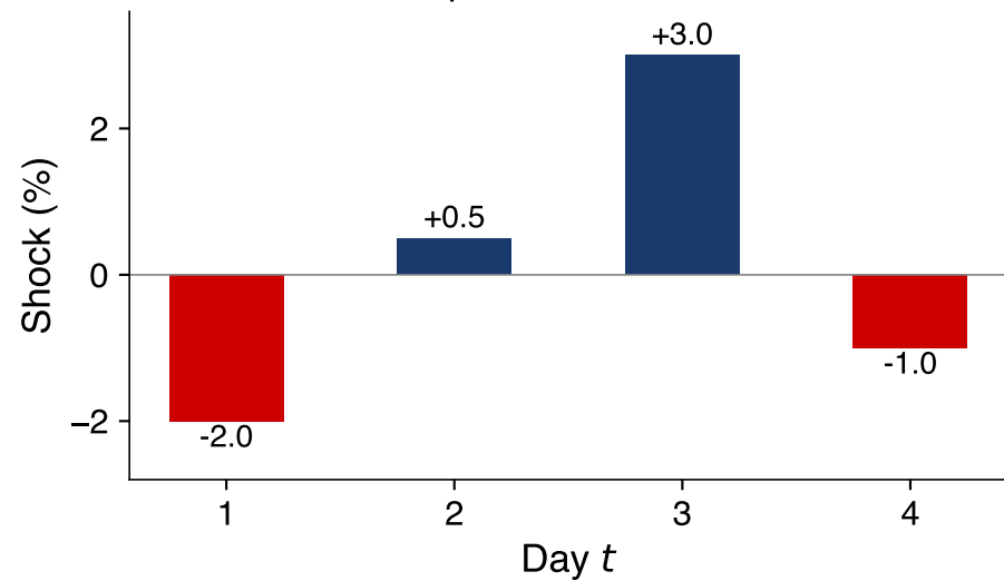
Input: four shocks
