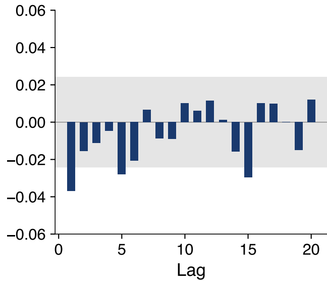
Autocorrelation
