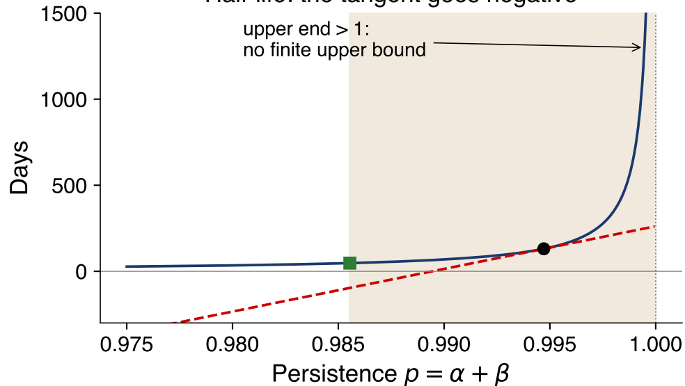
Half-life: the tangent goes negative
