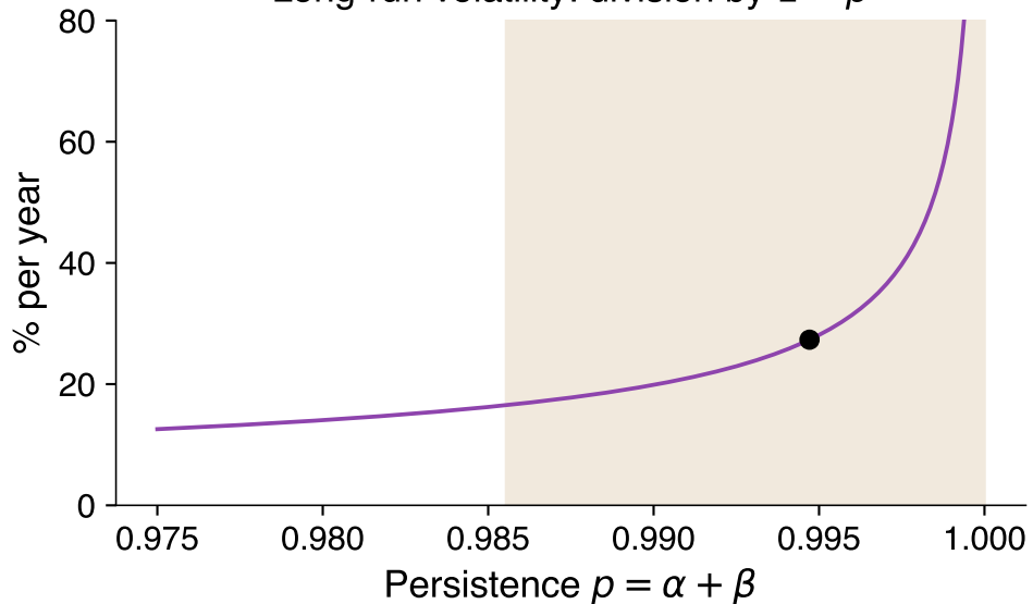
Long-run volatility: division by 1 - p
