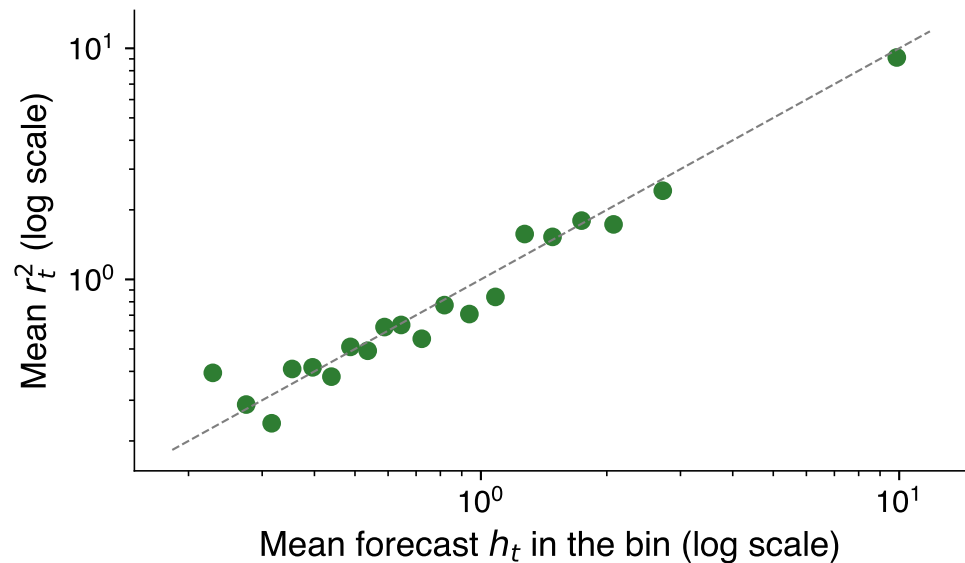
Binned calibration
