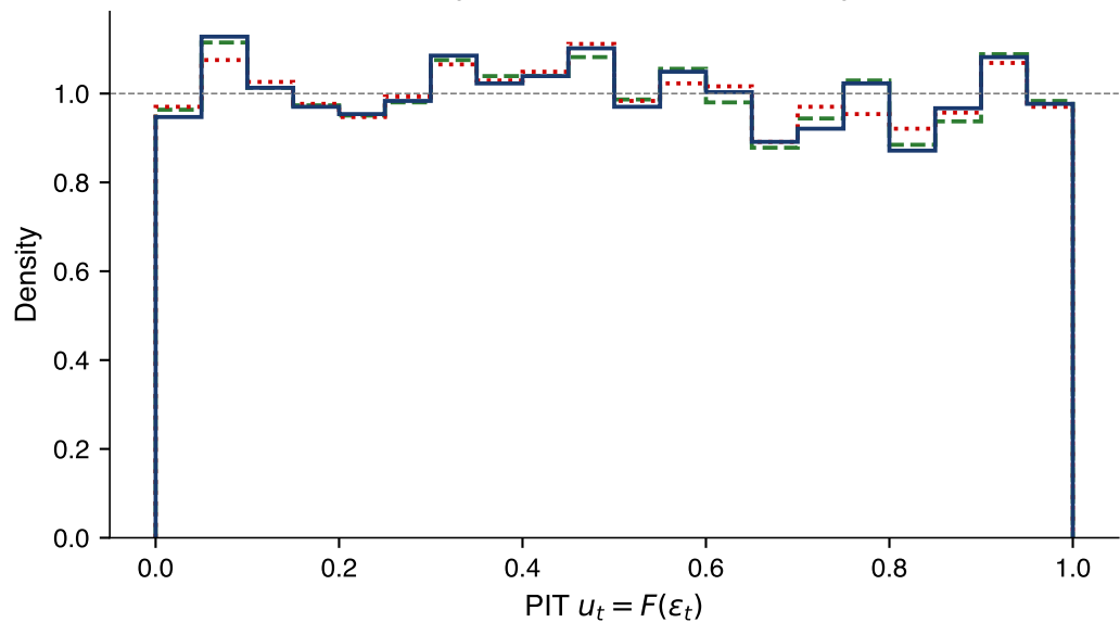
PIT histograms (uniform if the model is right)
