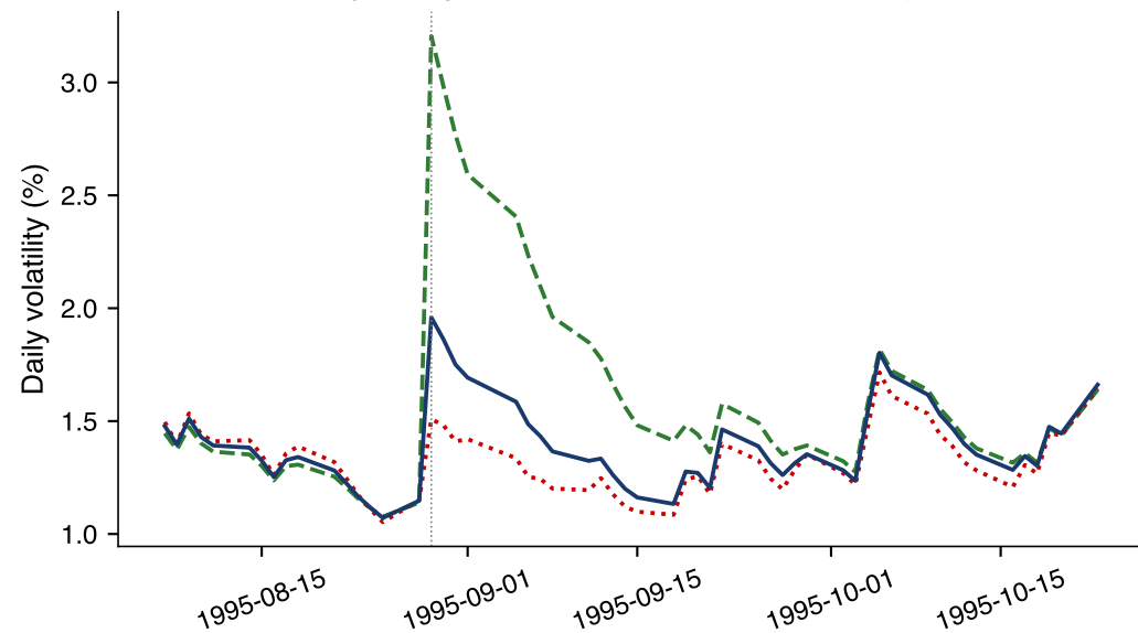
JPMorgan: largest shock on 1995-08-28 and the days after
