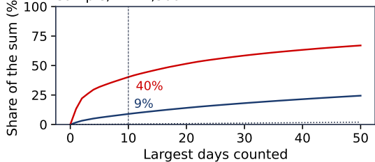
Sample, T = 2,500
