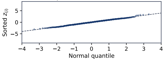
Normal sample
