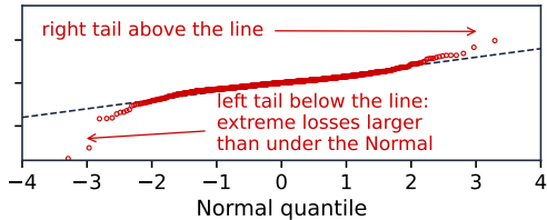
Student-t(3) sample
