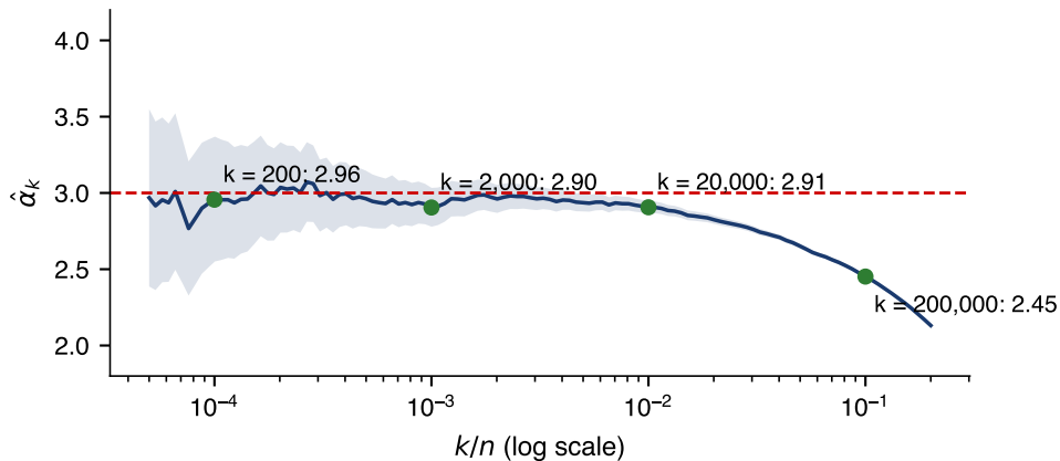
Hill estimates on 2,000,000 draws of |t_3| (seed 1)
