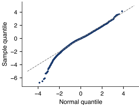
QQ plot vs the Normal distribution
