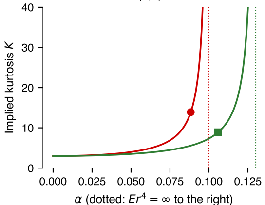
Gaussian GARCH(1,1): kurtosis vs \alpha
