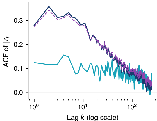
Around the CUSUM variance break
