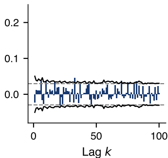
ACF of r_t
