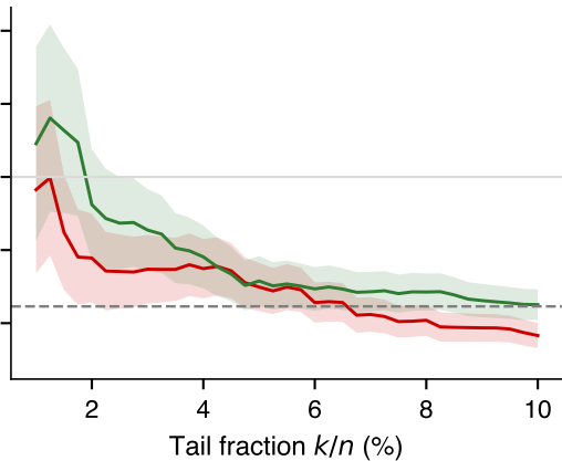
Bitcoin
