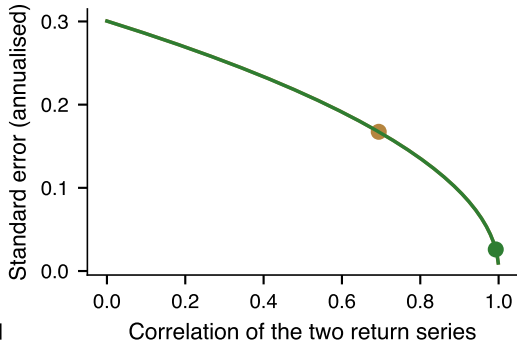
The standard error collapses as \rho \rightarrow 1
