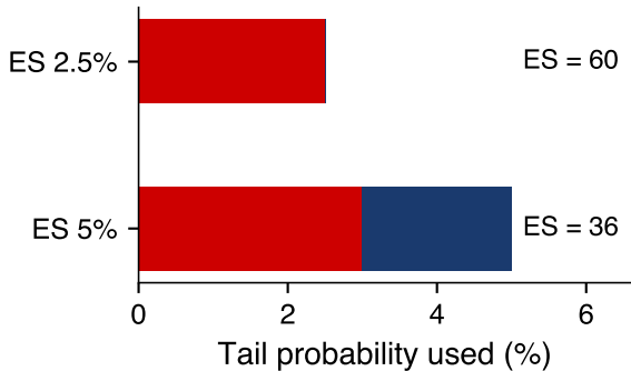
Probability mass in the worst \alpha of outcomes
