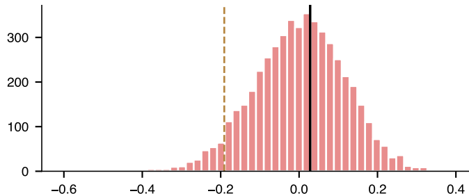
Bitcoin, GARCH-EVT: Z2 = 0.028 , p = 0.579
