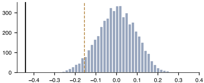
Bitcoin, GARCH-t: Z2 = -0.216 , p = 0.040
