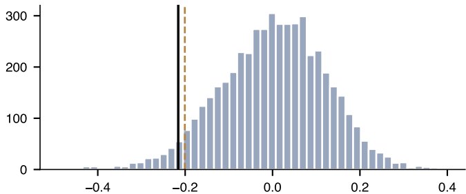
Bitcoin, GARCH-t: Z2 = -0.216 , p = 0.040
