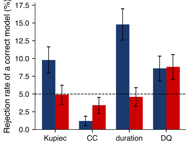
Size of the set of tests (bars: \pm 1.96 Monte Carlo standard errors)
