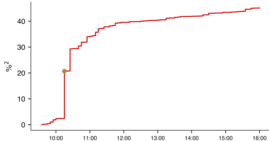
Realised variance accumulates over the day
