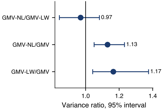
Paired block bootstrap
