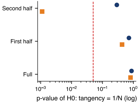
Three samples, two tests
