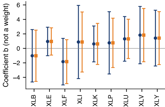
Full sample, T = 331
