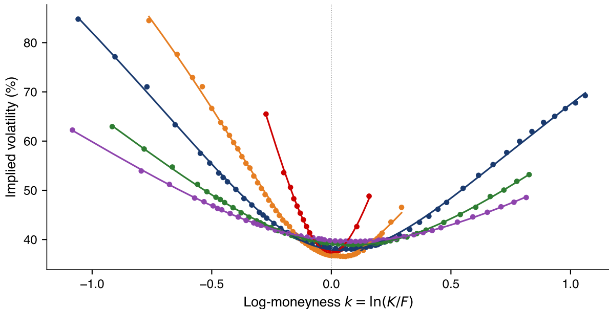
Bitcoin options, Deribit, 22 September 2026 07:51 UTC: quotes (dots) and SVI fits (lines)
