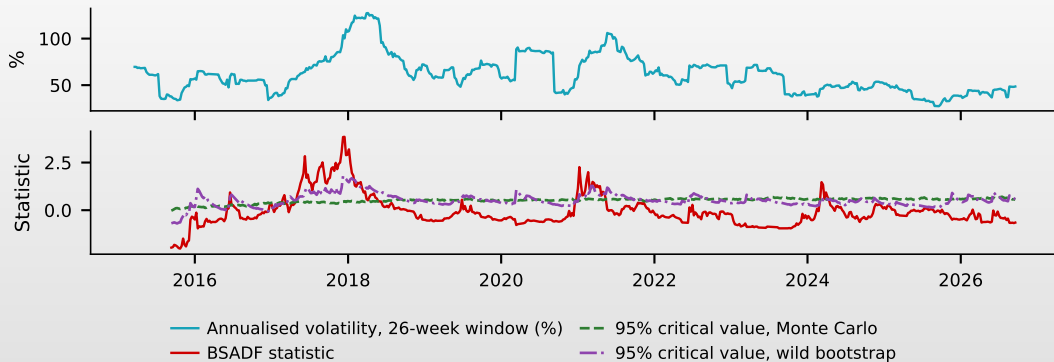
Bitcoin, weekly 2014-2026: volatility changes the critical values
