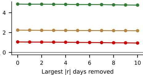
Crow-Siddiqui quantile kurtosis
