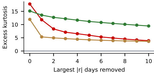
Moment excess kurtosis
