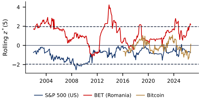
Time-varying efficiency: variance-ratio statistic on rolling 500-day windows
