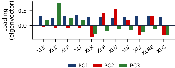
Loadings of the first three components
