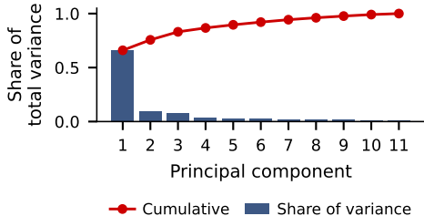
Scree plot
