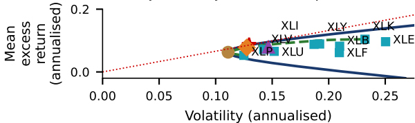
Nine sector ETFs, monthly excess returns Jan 1999 - Jul 2026 (in-sample)
