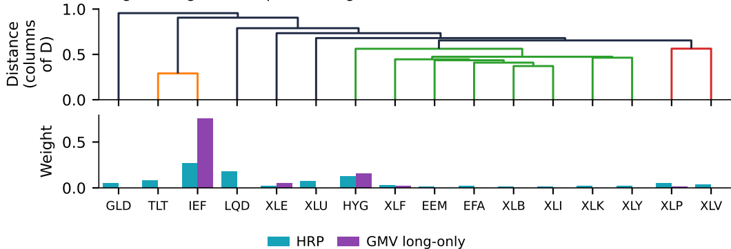
Single-linkage tree (top) and weights (bottom), same order of the assets
