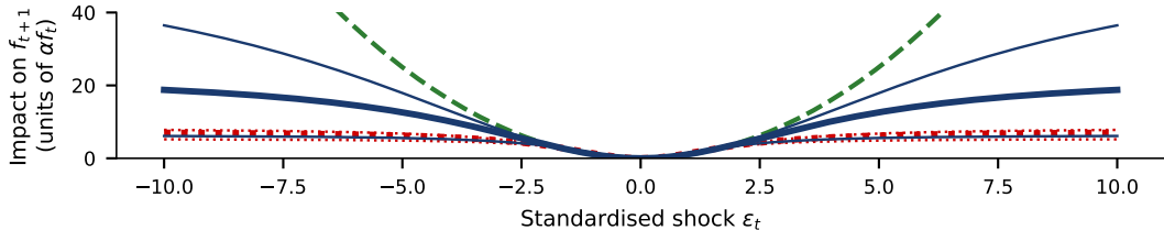
News impact curves, 11 S&P 500 stocks (quantiles over the stocks)
