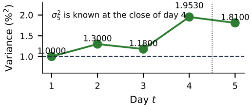
Output: \sigma_t^2 = \omega + \alpha \varepsilon_{t-1}^2 + \beta \sigma_{t-1}^2
