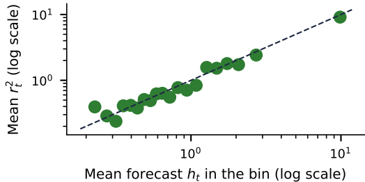
Binned calibration
