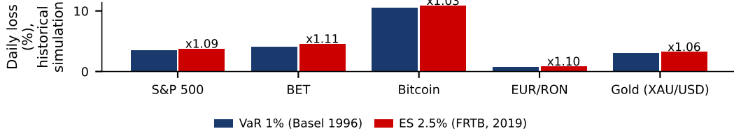
From VaR 1% to ES 2.5%: ratio ES/VaR above each pair
