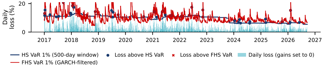
Bitcoin, 2017-2026: historical vs filtered historical simulation
