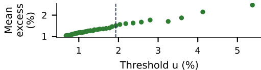
Mean excess plot
