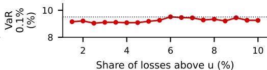
Extreme quantile vs threshold
