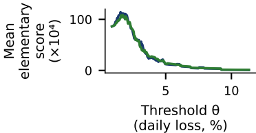
Murphy diagram, VaR 1%, S&P 500
