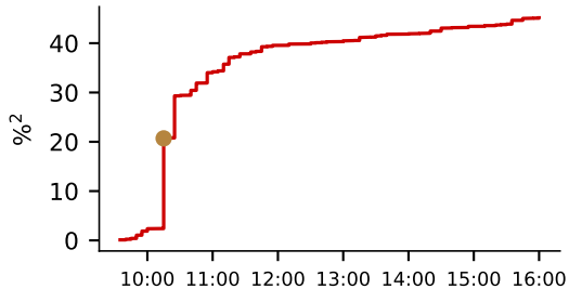
Realised variance accumulates over the day
