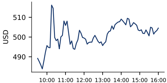
SPY on 7 April 2025
