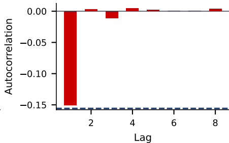
Only lag 1 is negative
