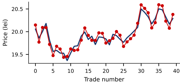
Simulated: trades alternate between bid and ask
