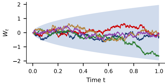
Five Brownian paths on [0, 1]
