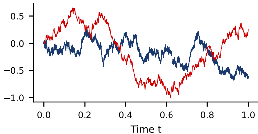
Self-similarity: zoom in and the path looks the same
