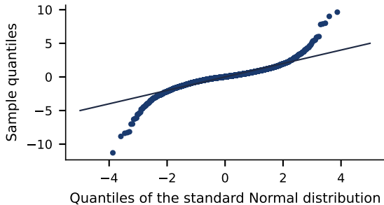
Tails: returns are not Normal
