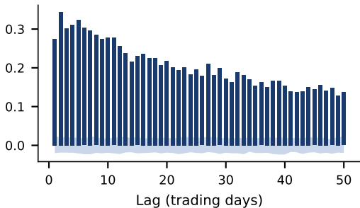
Clustering: |r| is autocorrelated
