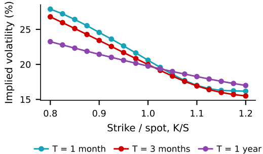
Fitted \rho = -0.69 : the skew flattens with maturity
