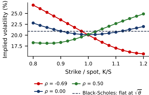
Three months: the sign of the smile follows \rho
