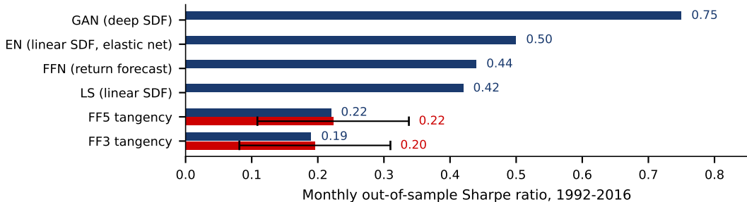
Deep SDF vs. benchmarks: monthly Sharpe ratio of the SDF portfolio, test 1992-2016
