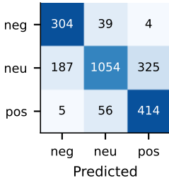
Qwen 7B: acc. 74.2%
