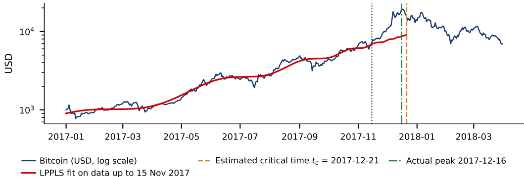
LPPLS on the 2017 Bitcoin bubble (search space of Shu and Zhu 2020, eq. 11)
