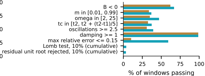
Filters of the confidence indicator
