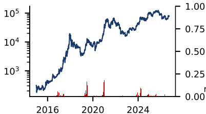
Bitcoin: LPPLS confidence indicator, 141 windows of 50-750 days, every 5 days
