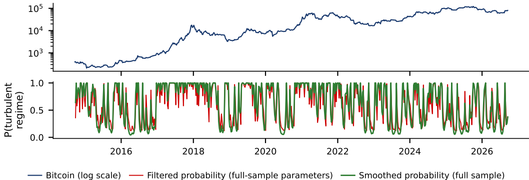
Bitcoin, weekly log returns 2014-2026: two-regime Markov-switching model
