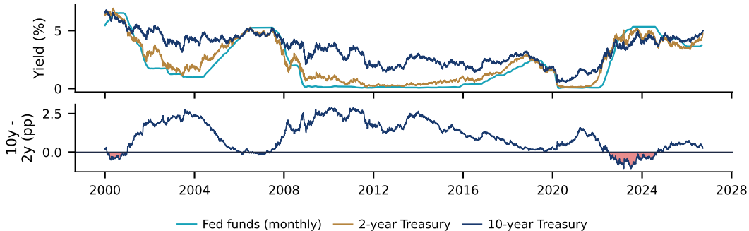
US rates and the 10y - 2y spread (red = inverted)
