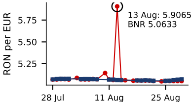
Level, Aug 2025
